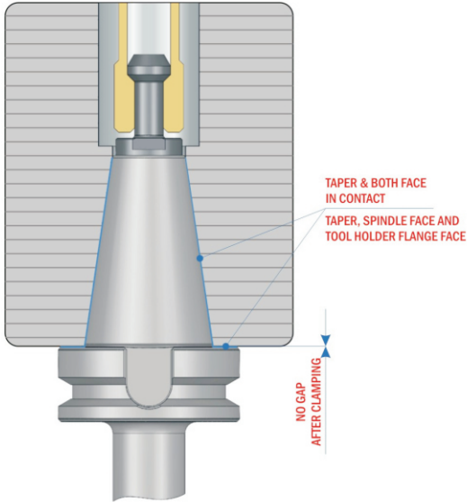
UBT (BT MAS 403) TAPER AND BOTH FACE CONTACT HOLDER (After Clamping)
